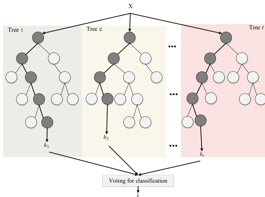
Figure 14. Random forest.
