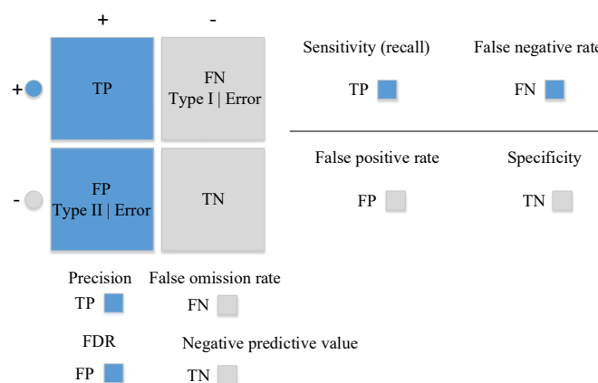
Figure 24. Confusion matrix.
