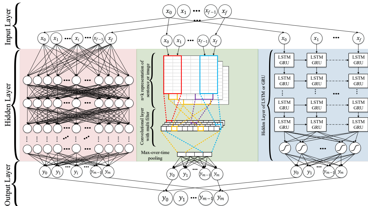
Figure 21. Random multimodel deep learning (RMDL) architecture for classification. RMDL includes 3 random models: A deep neural network (DNN) classifier ( left ), a deep CNN classifier ( middle ), and a deep recurrent neural network (RNN) classifier ( right ). Each unit could be a LSTM or GRU.
